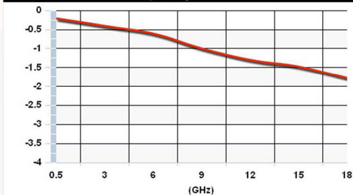
Insertion Loss vs. Frequency - 12 in. cable
