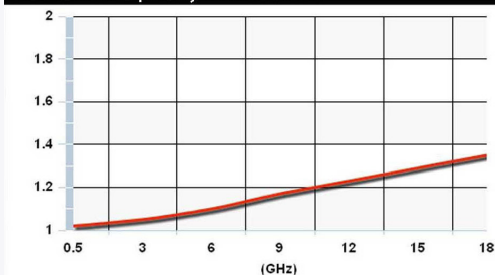
VSWR vs. Frequency - 12 in. cable
