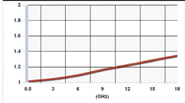
VSWR vs. Frequency - 12 in. cable
