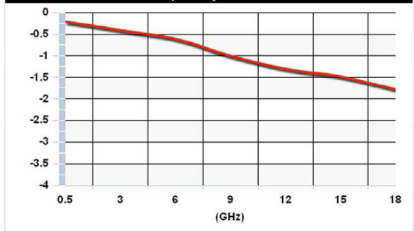
Insertion Loss vs. Frequency - 12 in. cable
