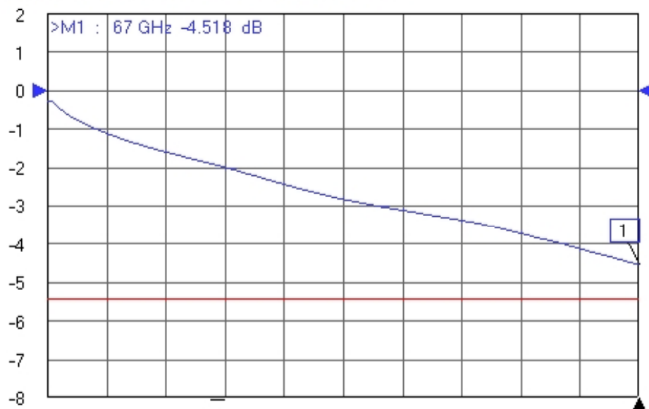
Tr3 S21 Trans LogM RefLvl: 0 dB Res: 1 dB/Div
