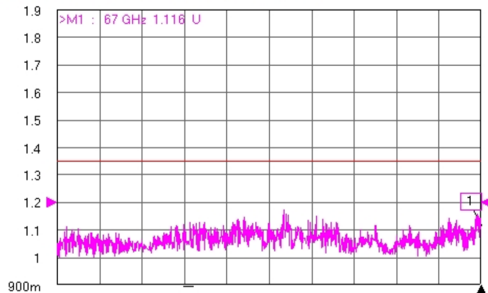
Tr4 S22 Refl SWR RefLvl: 1.2 U Res: 100 mU/Div
