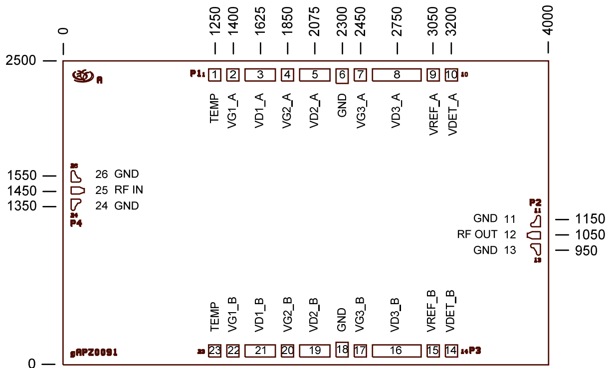
Figure 18. MMIC outline drawing
